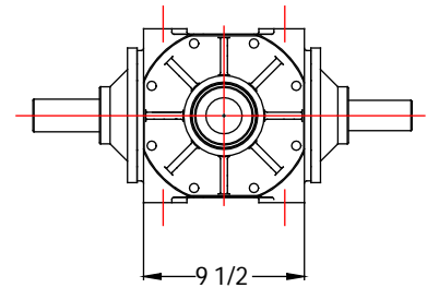
Top view 4X 5/8-11 NC ON BOTH SIDES
